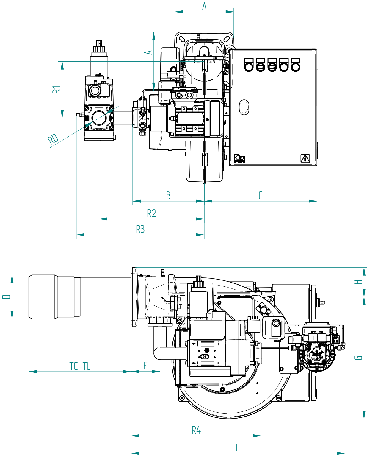
Fig. 3 Dimensions: K 4/2 EVO 2
